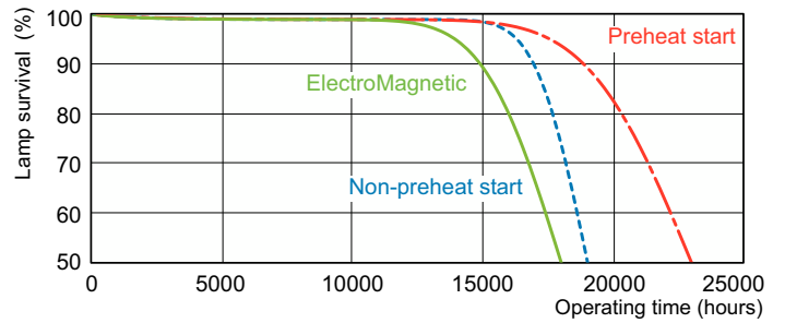
Life Expectancy Diagram - MST TL-D Reflex 18W/840 1 SLV/25
